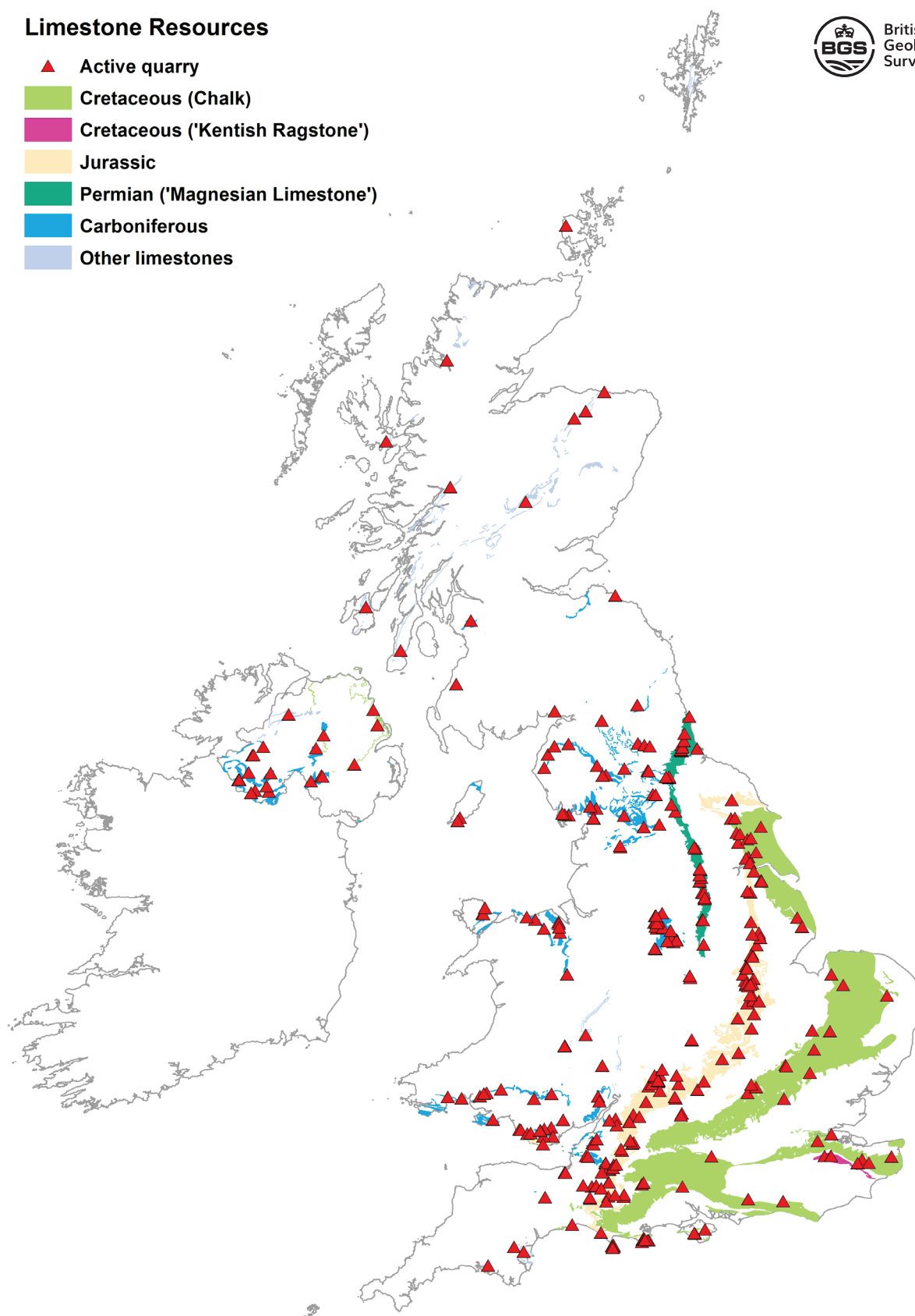
Figure 4 Limestone resources and workings in the UK in 2020.
