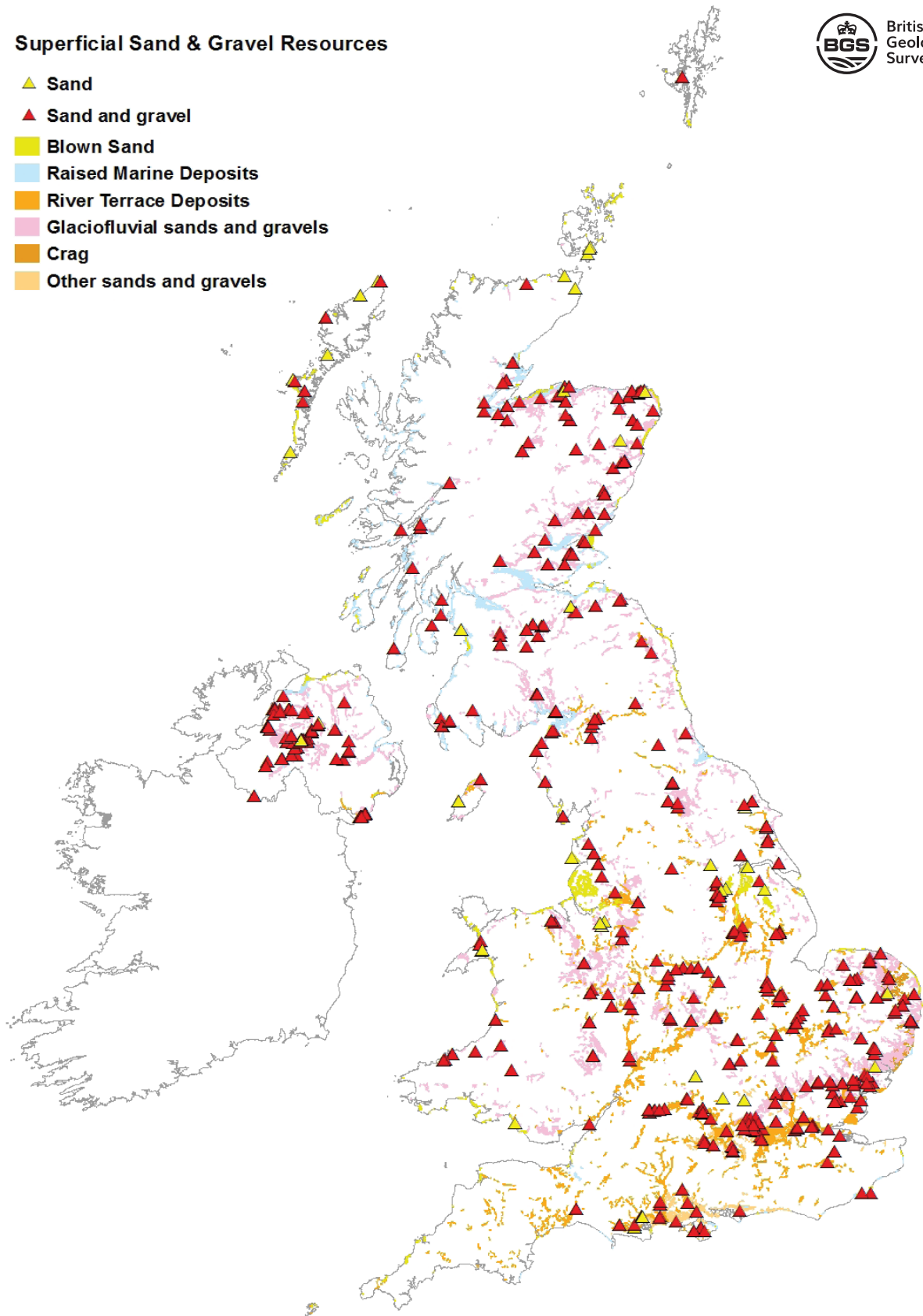
Figure 5 Sand & Gravel resources and workings in the UK in 2020; see Figure 11.
