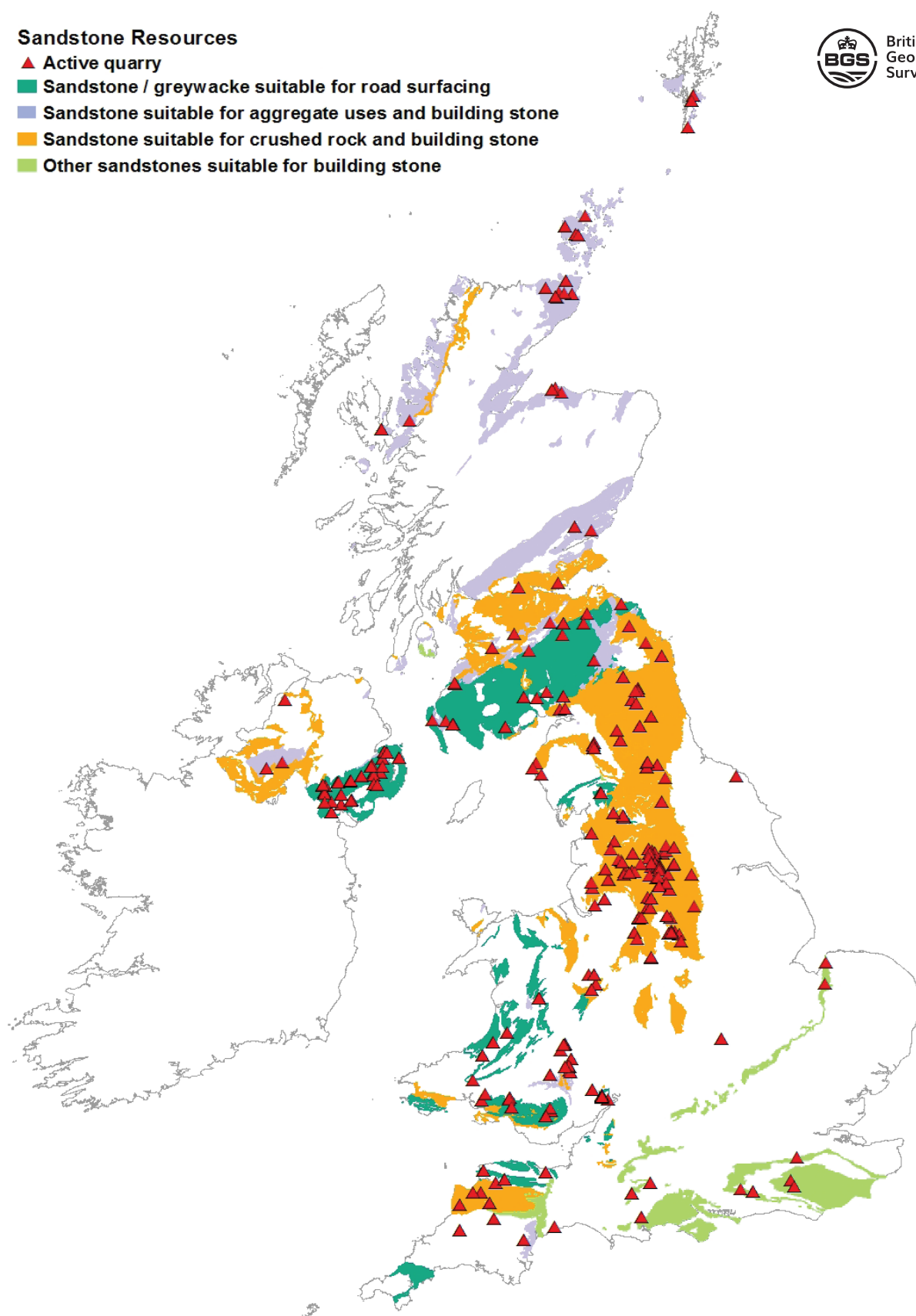
Figure 7 Sandstone resources and workings in the UK in 2020.
