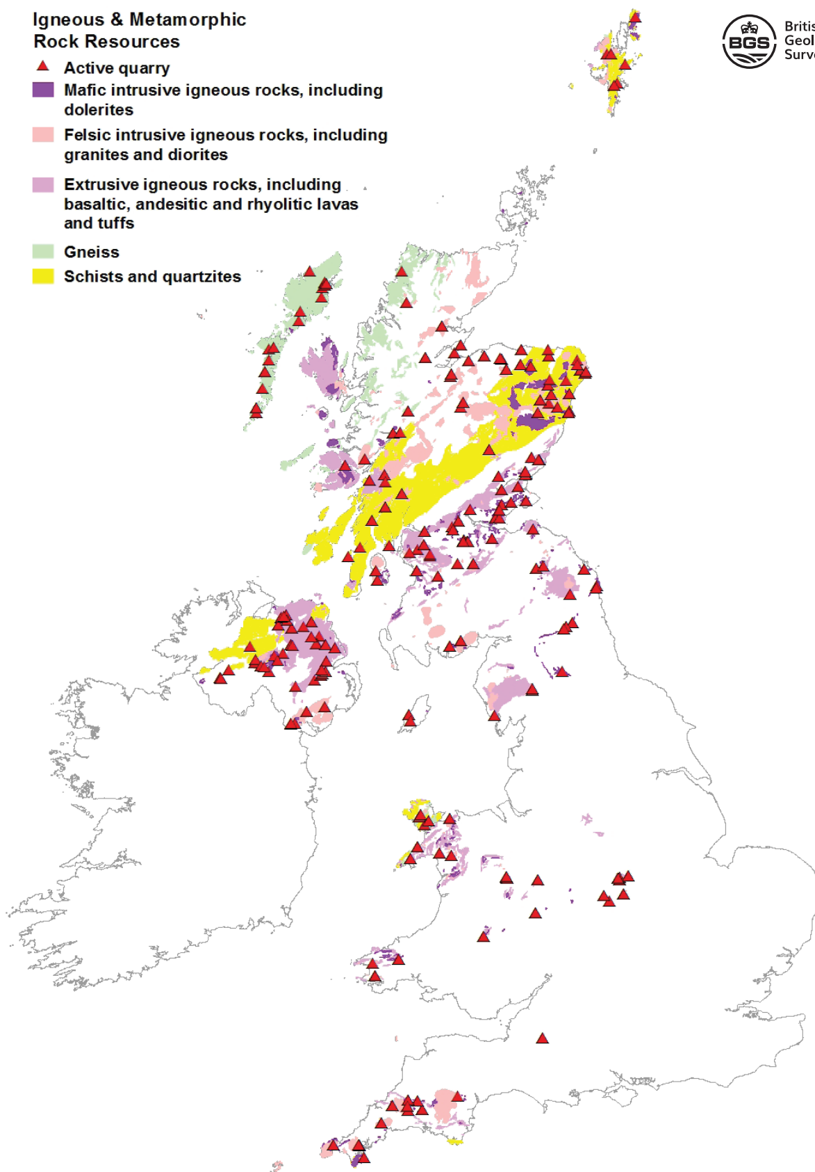
Figure 3 Igneous & Metamorphic Rock resources and workings in the UK in 2020.
