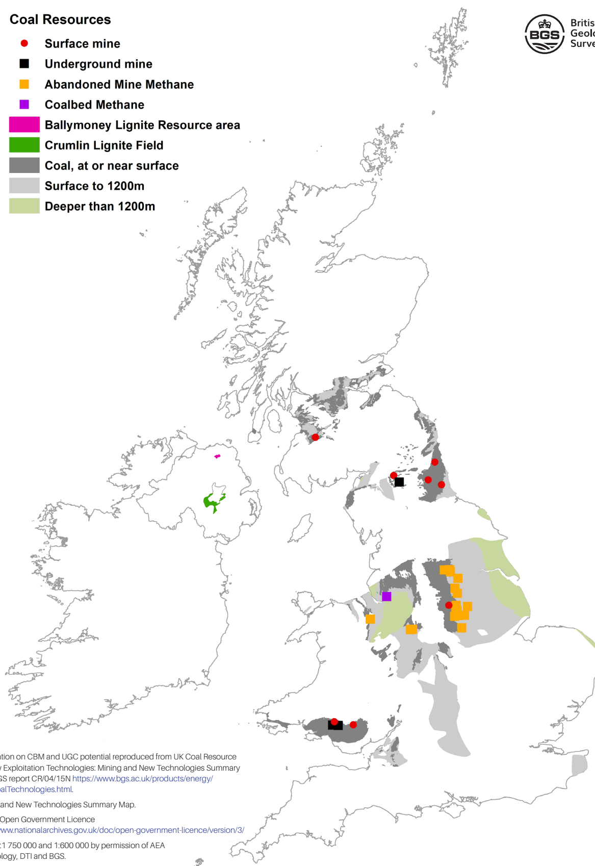
Figure 8 Coal resources and workings in the UK in 2020.
