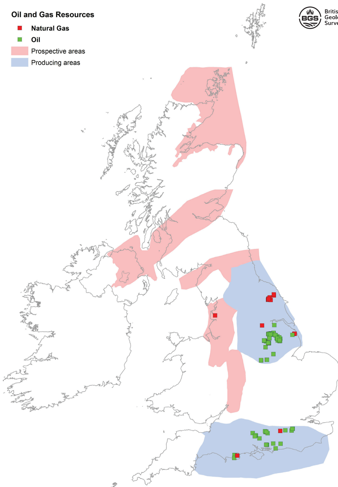
Figure 9 Oil and gas resources and workings in the UK in 2020.
